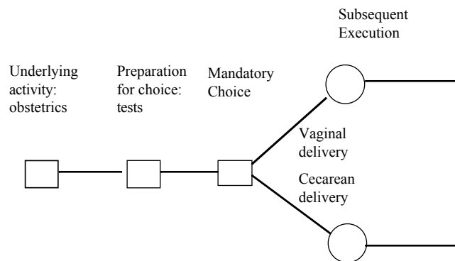
Figure 2: Acts Preceding and Following a Mandatory Choice
